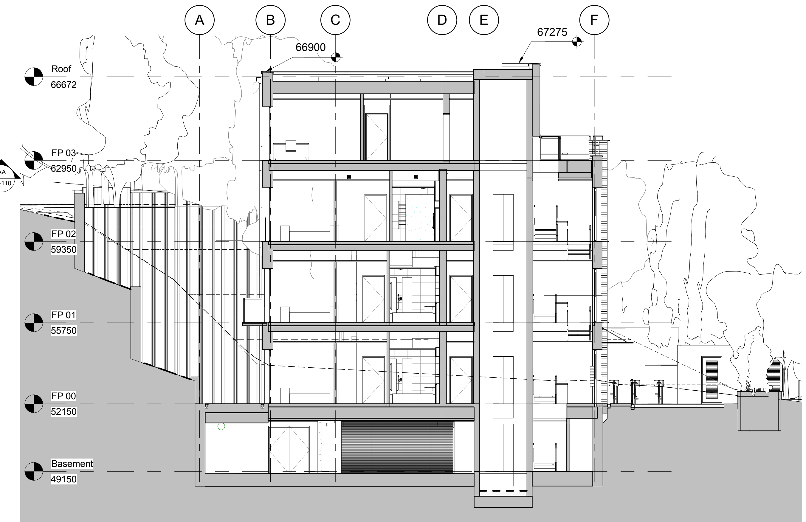
AA LEVEL SECTION 1:100
